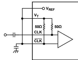
CONNECT V_T , V_{REF} , AND \overline{\text{CLK}} . PLACE A BYPASS CAPACITOR FROM V_T TO GROUND. ALTERNATIVELY, V_T , V_{REF} , AND CLK CAN BE CONNECTED, GIVING A CLEANER LAYOUT AND A 180° PHASE SHIFT. Figure 22. Interfacing to AC-Coupled Single-Ended Inputs
